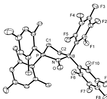
Figure 1. X-ray structure of P/B-FLP-NO ( 3 ). [33]
