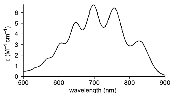
Figure 3. Visible spectrum of P/B-FLP-NO \cdot ( 3 ) in fluorobenzene at room temperature.
