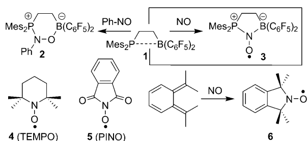
Scheme 1. Synthesis of P/B-FLP-NO ( 3 ) with related N-oxyl radicals.
