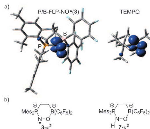
Figure 4. a) Spin density plot of 3 and TEMPO (isospin = 0.001). b) Alternative structures considered for 3 and 7 with P–N–O–B linkages.
