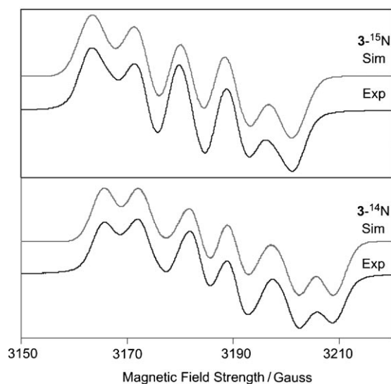
Figure 2. X-band EPR spectra (fluorobenzene, room temperature) and simulations for P/B-FLP-NO \cdot ( 3 - ^{14}\text{N} , bottom; 3 - ^{15}\text{N} , top).
